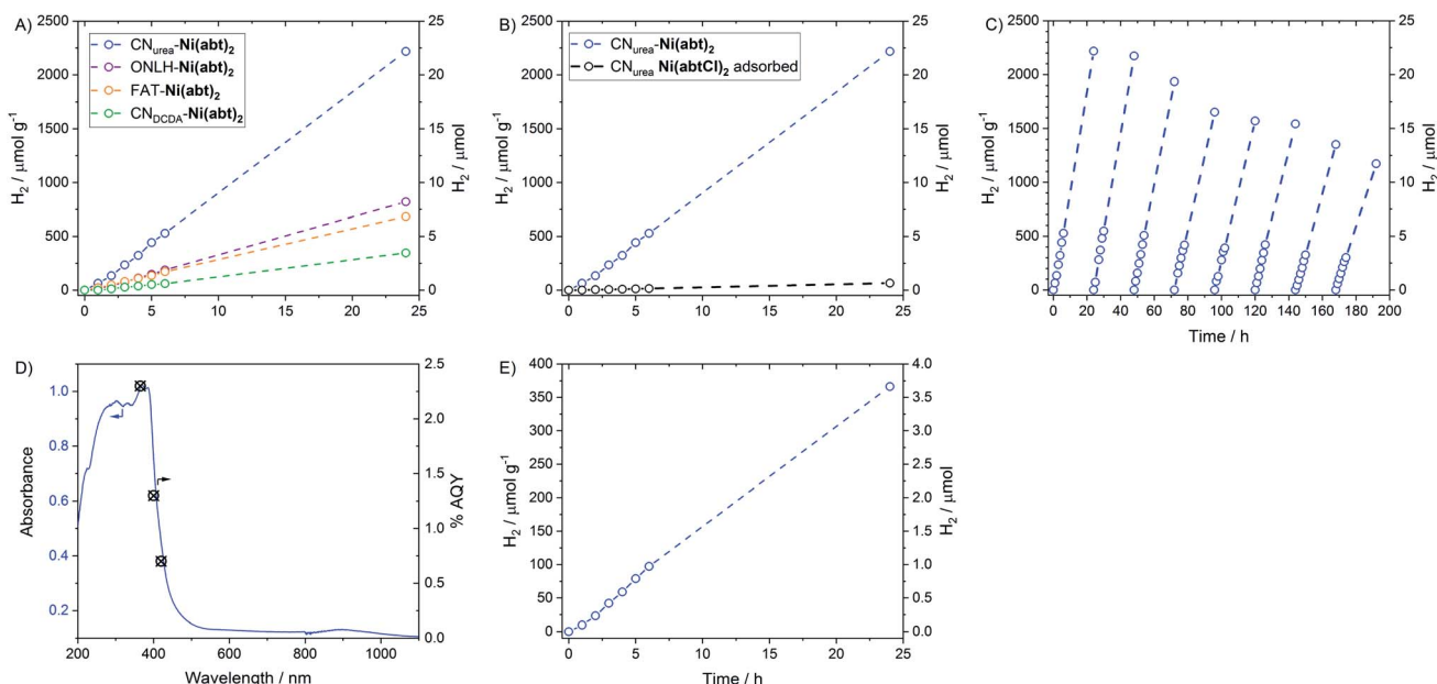
Fig. 4 Photocatalytic hydrogen production by (A) CN-Ni(abt) 2 hybrids (B) CN urea -Ni(abt) 2 compared with CN urea with Ni(abtCl) 2 adsorbed (C) CN urea -Ni(abt) 2 activity for 8 days (D) quantum yields of H 2 overlaid with DRUVS spectrum for CN urea -Ni(abt) 2 . All in H 2 O with 10% TEOA and λ > 420 nm (pH = 11). (E) ONLH-Ni(abt) 2 with λ > 475 nm.
