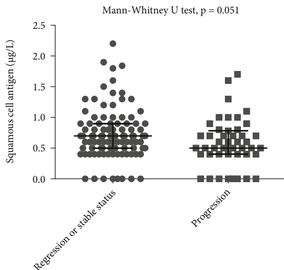
FIGURE 1: Concentration of SCCA in patients with regression/stable status and progressed status.
