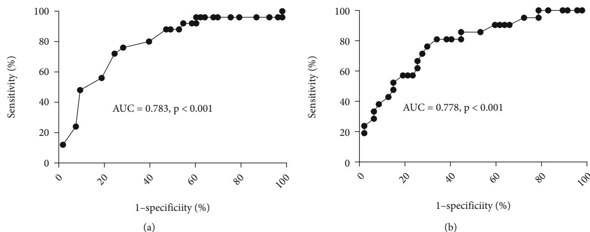
FIGURE 2: A receiver operating characteristic curve between predictive probability and progression of mild/moderate dysplasia of the esophagus mucosa. (a). Males and (b) females.
