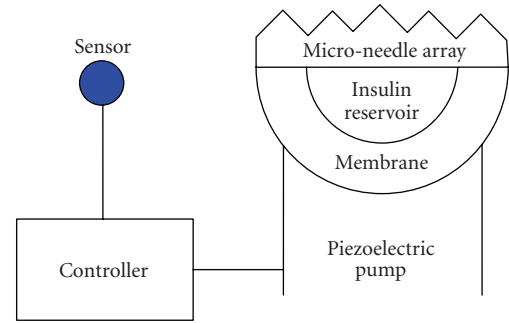
FIGURE 4: Piezoelectric pump and micro-needle device.
