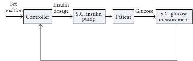
FIGURE 10: A control flow of closed-loop control models [15]. Entire loop of the control is closed from outside by utilizing an insulin pump and in vivo blood glucose sensors. Both insulin injections and glucose measurements are carried out subcutaneously.
