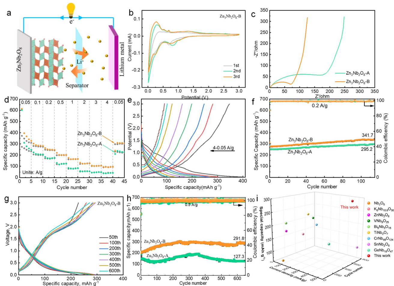
Fig. 4 (a) Schematic illustration of Zn 3 Nb 2 O 8 /Li lithium-ion cell. (b) CV curves of Zn 3 Nb 2 O 8 -B at the scan rate of 0.1 mV s -1 ; (c) Nyquist plots of Zn 3 Nb 2 O 8 -A and Zn 3 Nb 2 O 8 -B; (d) rate performances of Zn 3 Nb 2 O 8 -A and Zn 3 Nb 2 O 8 -B at different current densities; (e) galvanostatic discharge and charge curves of Zn 3 Nb 2 O 8 -B at different current densities from 0.05 to 4.0 A g -1 . (f) Cycling performances of Zn 3 Nb 2 O 8 at a current density of 0.2 A g -1 ; (g) discharge and charge curves of Zn 3 Nb 2 O 8 -B at a current density of 0.5 A g -1 ; (h) cycling performances of Zn 3 Nb 2 O 8 at a current density of 0.5 A g -1 . (i) Comparison of cycling stability between Zn 3 Nb 2 O 8 -B with other Nb-based anode materials.
