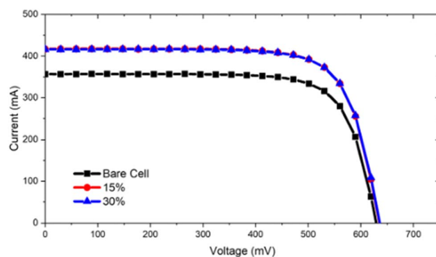
Fig. 3 I - V curves obtained under the irradiation of standard AM1.5G for cells with LDSLs containing different concentrations of \text{Eu}(\text{DPIQC})_3 in PVB.
