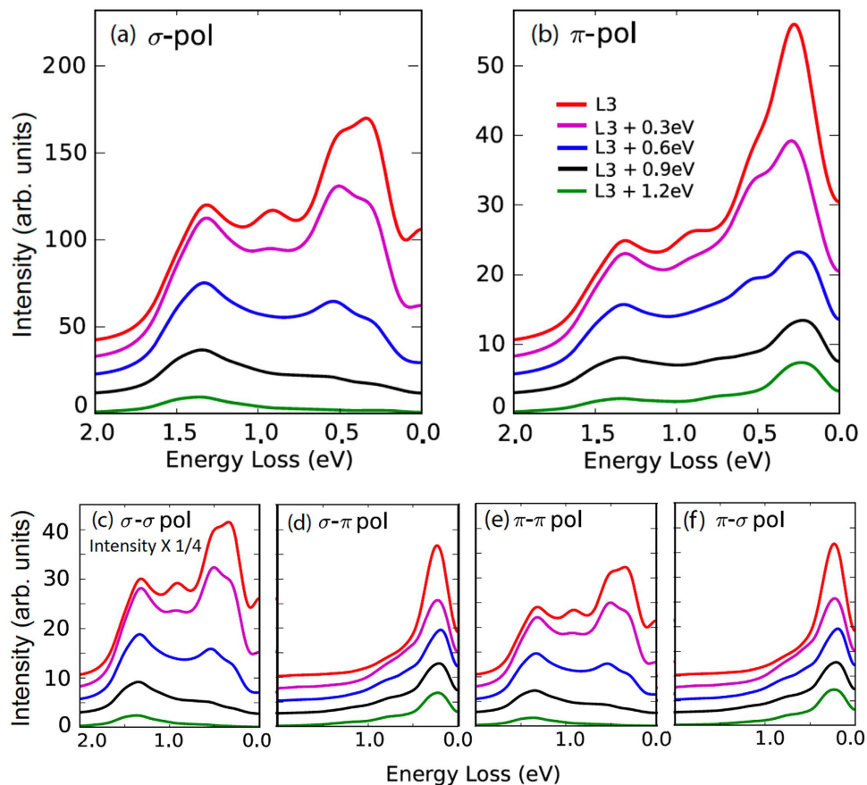
Figure 3. Full RIXS ED calculations. The ED calculations were performed as described in Methods using the single-band Hubbard model on a 12-site cluster under TABC (100 boundary conditions were used) at 16.7% hole-doping. The parameter values are given in Methods. Panel (a) and (b) show the calculated spectra for \sigma -incoming polarization and \pi -incoming polarization respectively. Panel (c) through (f) show the calculated spectra also discriminating the outgoing photon polarization, which are plotted on the same linear intensity scale (intensity of Fig. 3(c) is multiplied by 1/4). For all panels an offset is used for clarity. The transferred momentum is (2\pi/3, 0) for \sigma -polarization incidence and (-2\pi/3, 0) for \pi -polarization incidence in theory units where the lattice constant a is 1.
