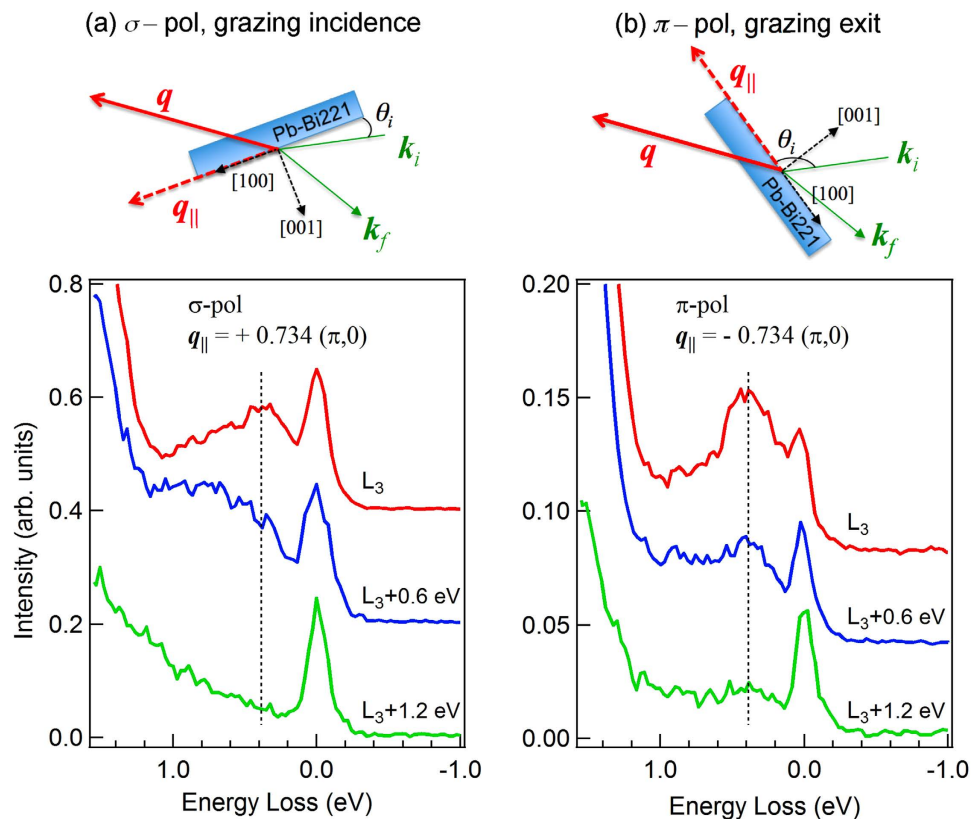
Figure 2. Magnified plots of RIXS excited with X-rays at selected energies. (a,b): RIXS spectra taken with \sigma -polarized incident X-rays under a grazing-incidence geometry and \pi -polarized incident X-rays under a grazing-exit geometry, respectively. The RIXS spectra of each scattering geometry are normalized to the elastic scattering of energy set to the L_3 absorption threshold. The RIXS spectra are vertically offset for clarity. Top panels illustrate the scattering geometries in which the scattering plane is defined by the [001] & [100] of the Pb-Bi2212 crystal. All notations are defined in Fig. 1. The dashed lines serve as guides to the eyes.
