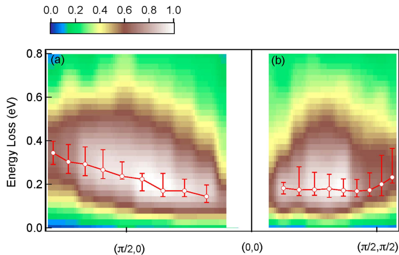
Figure 4. Intensity maps of magnetic RIXS and dispersion of magnetic excitations in Pb-Bi2212. The momentum transfer \mathbf{q}_{\parallel} is varied along (0, 0) \rightarrow (\pi, 0) in panel (a) and (0, 0) \rightarrow (\pi, \pi) in panel (b). The RIXS intensities shown in the color maps are after background subtraction. The excitation energies shown in red open circles are deduced from RIXS data with \pi -polarized incident X-rays as described in the text.
