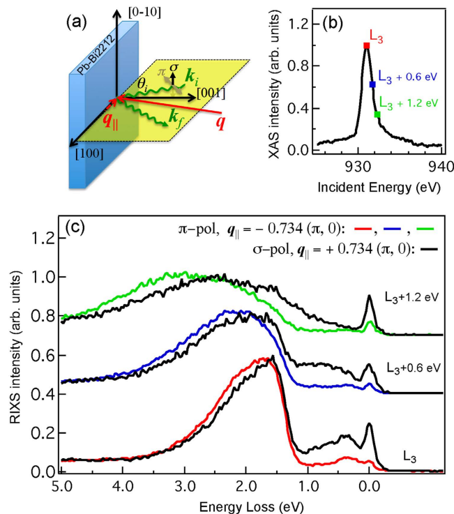
Figure 1. RIXS spectra of Pb-Bi2212. (a) RIXS scattering geometry. The angle between the incident X-ray and the ab plane of the sample is \theta_i . The wave vectors of incident and scattered X-rays are k_i and k_f , respectively. The momentum transfer is \mathbf{q} = k_i - k_f , and its projection onto the ab plane is q_{\parallel} . (b) Cu L_3 -edge X-ray absorption (XAS) measured in the fluorescent yield mode. The energy bandwidth of incident X-ray is 0.6 eV. (c) RIXS spectra with incident X-ray energy set to the L_3 absorption threshold, 0.6 eV above, and 1.2 eV above using \pi -polarized (color) and \sigma -polarized (black) X-rays with \theta_i = 110^\circ and 20^\circ , i.e. grazing-exit q_{\parallel} = -0.734(\pi, 0) and grazing-incidence q_{\parallel} = 0.734(\pi, 0) , respectively. Spectra are normalized to the dd excitations and also offset for clarity.
