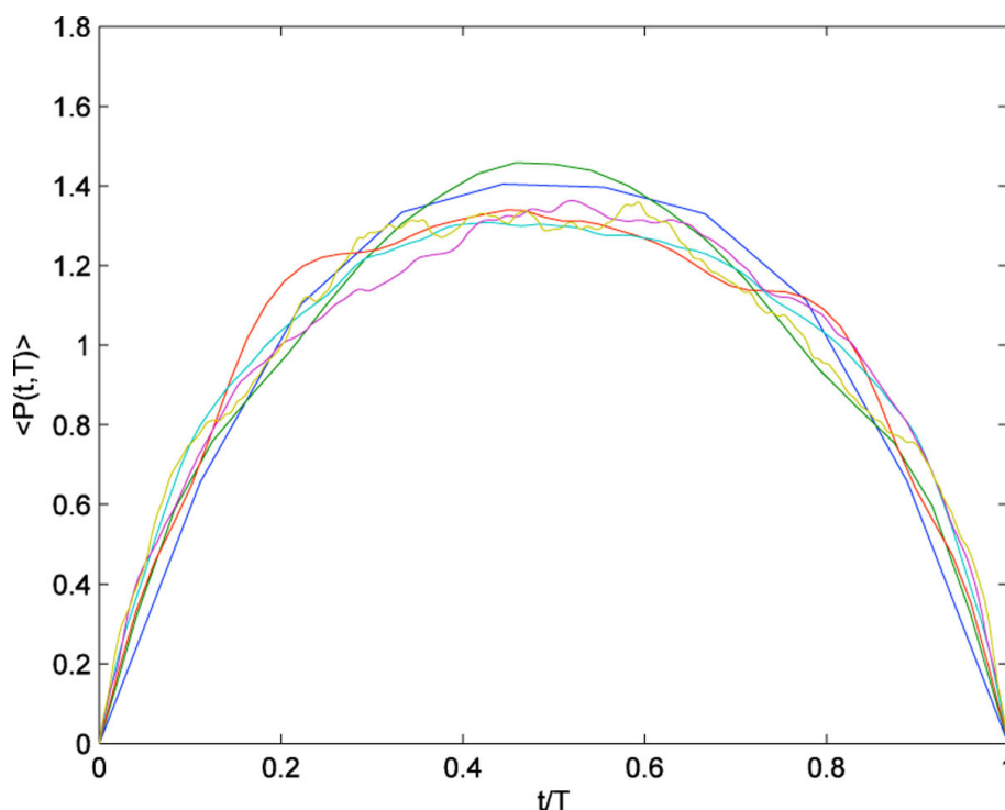
Figure 1 Example of single-subject average burst shapes collapsing to a simple symmetric functional form over temporal scales of T = 40 \text{ ms} - 4 \text{ s} .
