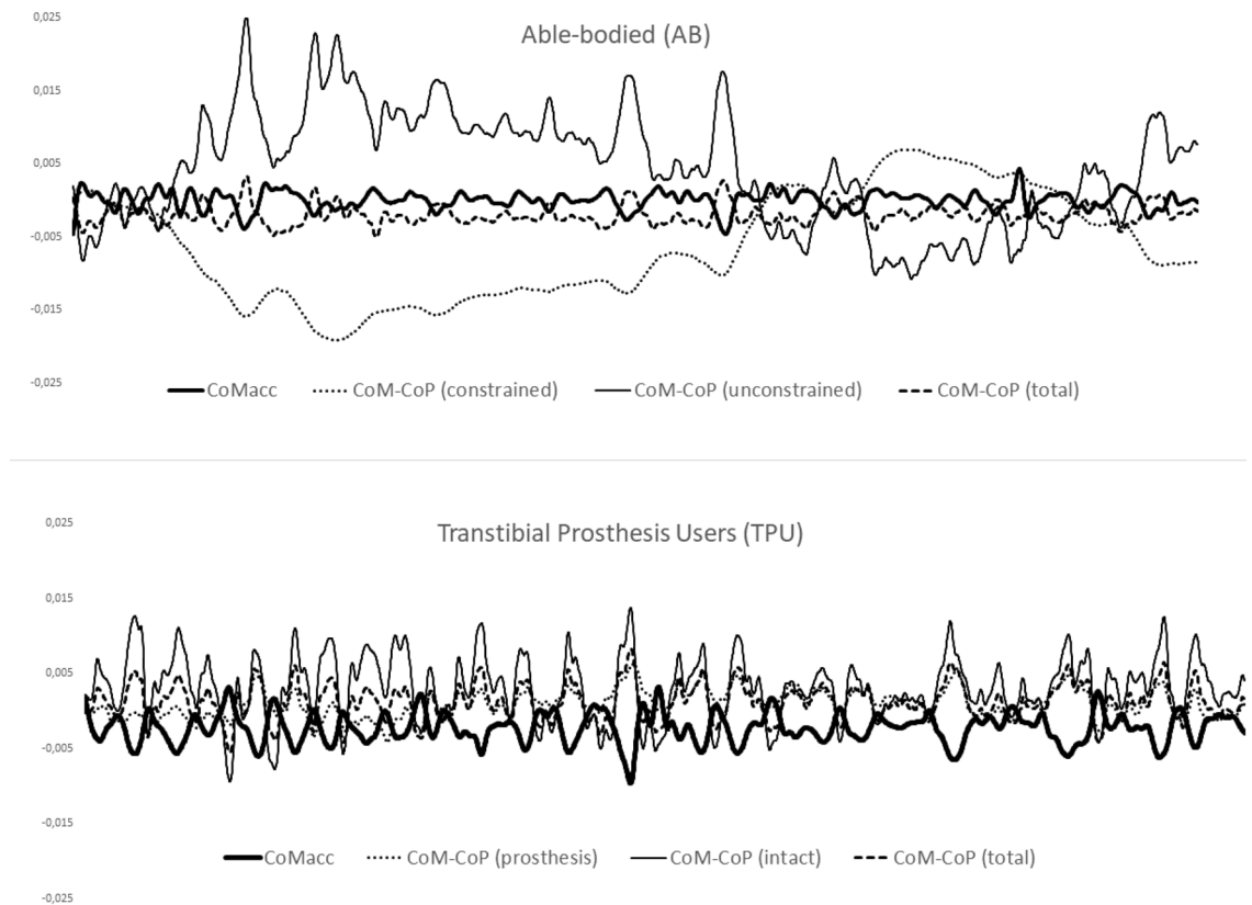
Figure 2. 30-s representative time curve for the sagittal plane (anteroposterior) for the able-bodied group (AB) and the transtibial prosthesis user group (TPU). Outcomes in the curve are centre of mass acceleration ( CoM_{Acc} ), difference between the position of the centre of mass and centre of pressure (CoM-CoP) for each of the three sides of interest (prosthetic limb/constrained for AB group), intact limb/unconstrained for AB group, and total). Given the coordinate system utilized (positive = anterior), negative values indicate the CoM is posterior to the CoP.
