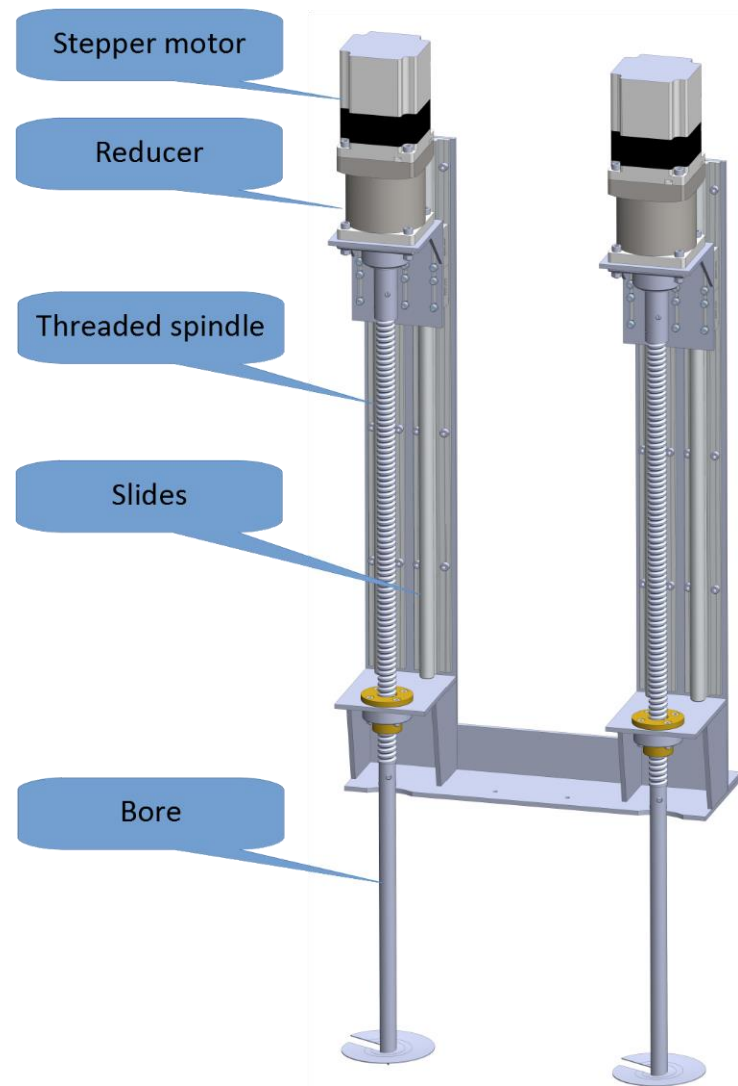
Figure 5. Model of the anchoring module.
