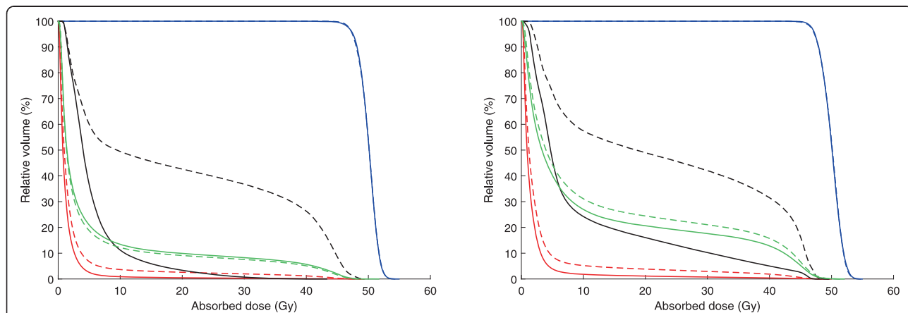
Figure 2 Mean dose volume histograms. Mean dose volume histograms for tangential treatment (left) and locoregional treatment (right) comparing EIG (solid lines) and FB (dashed lines) for LAD (black), heart (red), ipsilateral lung (green) and PTV (blue).
