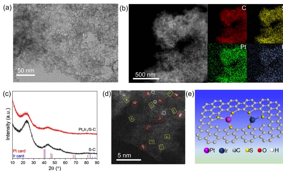
Fig. 2 Characterization of the atomically dispersed \text{Pt}_1\text{Ir}_1/\text{S-C} catalyst. TEM (a) and (b) HAADF-STEM images of \text{Pt}_1\text{Ir}_1/\text{S-C} . (c) XRD curves of S-C and PtIr/S-C. (d) Atomic-resolution HAADF-STEM image of \text{Pt}_1\text{Ir}_1/\text{S-C} , where representative isolated atoms (Pt or Ir), dimers, and clusters are highlighted by white circles, yellow rectangles, and red squares, respectively. (e) Schematic of the \text{Pt}_1\text{Ir}_1 pair over the S-C support.
