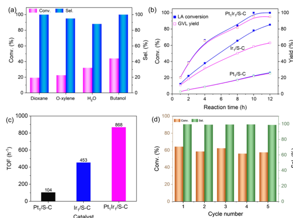
Fig. 4 Catalytic performance for the hydrogenation of LA. (a) Hydrogenation of LA over the Pt 1 Ir 1 /S-C catalyst in different solvents. Reaction condition: 5 mg Pt 1 Ir 1 /S-C catalyst, 1 mmol LA, 3 mL solvent, 180 °C, 4 MPa H 2 , and 4 h. (b) Reaction kinetics over Pt 1 Ir 1 /S-C, Pt 1 /S-C, and Ir 1 /S-C catalysts. (c) Activity of different catalysts for the hydrogenation of LA. (d) Recycling of Pt 1 Ir 1 /S-C for phenylacetylene semihydrogenation within 4 h. Reaction conditions: 1 mmol LA, 3 mL butanol, 180 °C, 4 MPa H 2 , and 4 h.
