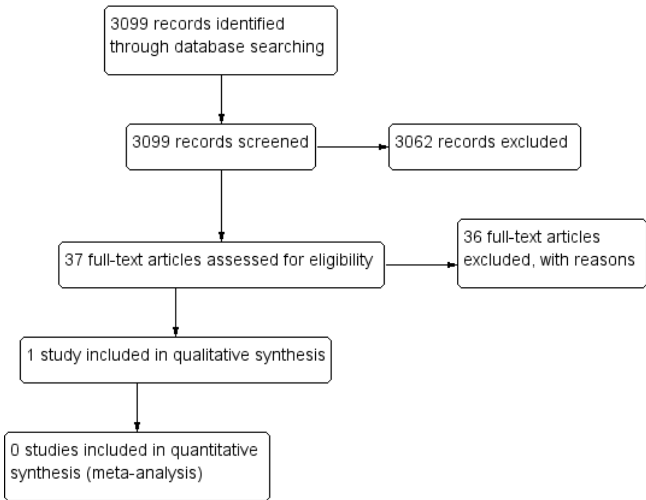
Figure 2. PRISMA diagram.
