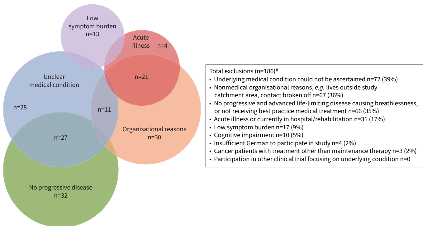
FIGURE 4 Reasons for exclusion. Minor overlaps in Venn diagram are not reported. Venn diagram: https://www.biovenn.nl/ . #: multiple answers possible.
