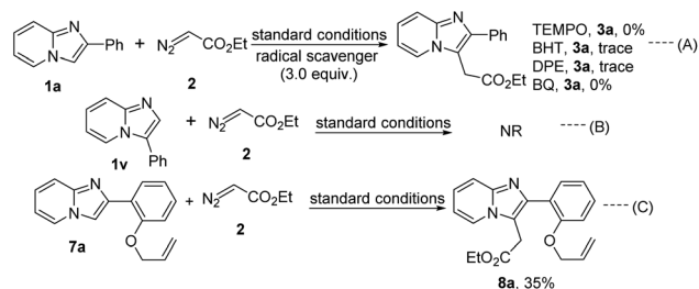
Scheme 4 Control experiments.
