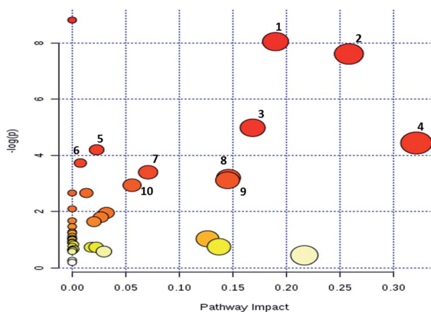
Fig. 6 Differentially regulated metabolic pathway analysis of MM serum metabolites. Metabolic pathway map of differentially regulated metabolites generated using MetPa tool of MetaboAnalyst web application. Significant pathways identified includes (1) pyrimidine metabolism, (2) alanine, aspartate and glutamate metabolism, (3) glycine, serine and threonine metabolism, (4) cysteine and methionine metabolism, (5) purine metabolism, (6) nitrogen metabolism, (7) sulfur metabolism, (8) citrate cycle (TCA cycle), (9) riboflavin metabolism (10) pentose and glucuronate interconversions.
