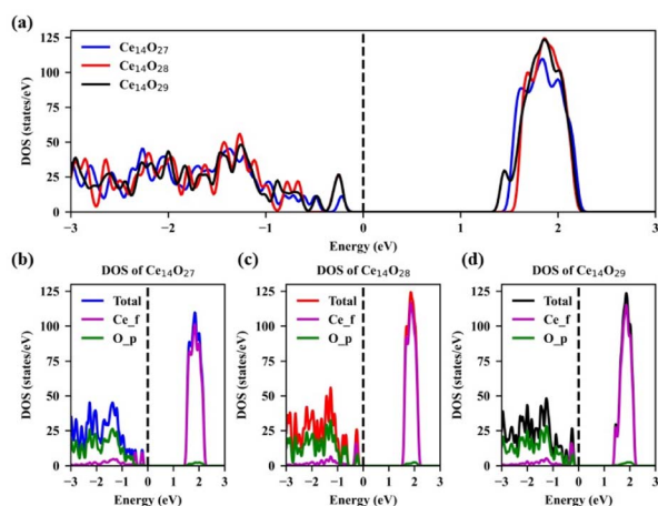
Fig. 7 Density of states (DOS) of the most stable structures of Ce 14 O x ( x = 27, 28, and 29 ): (a) TDOS of Ce 14 O x ( x = 27, 28, and 29 ); (b) DOS of Ce 14 O 27 ; (c) DOS of Ce 14 O 28 ; (d) DOS of Ce 14 O 29 .
