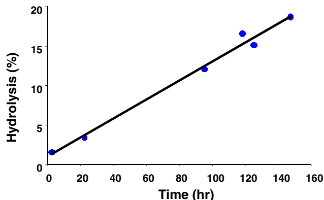
Fig. 8 Hydrolysis of RFK peptide from D10PS-RFK-FITC nanoparticles over time.
