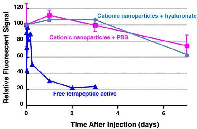
Fig. 9 In vivo pharmacokinetics of 37.5:37.5:25 D10P:D20P-VivoTag: Eudragit RL100 nanoparticles coinjected with PBS or hyaluronate versus free tetrapeptide in PBS.
