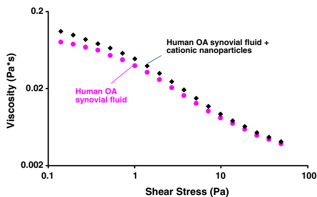
Fig. 5 Viscosity as a function of shear stress of human OA synovial fluid alone and treated with cationic 75:20:5 D10P:Eudragit RL100:MEH-PPV nanoparticles.
