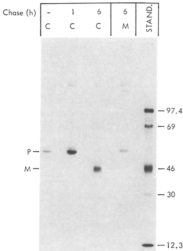
Figure 2. Molecular forms of cathepsin D in rat hepatoma (Morris hepatoma 7777) cells. Morris hepatoma 7777 cells were labeled for 10 min with [ 35 S]methionine and harvested after a chase for up to 6 h. Cathepsin D was immunoprecipitated from extracts of cells (C) and medium (M). The precursor (P) and mature (M) forms of cathepsin D are indicated. For standards see Fig. 1.
