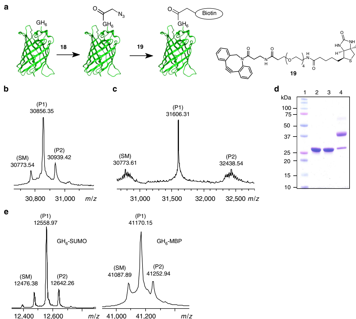
Fig. 4 Functionalization of proteins with azides, biotin and PEG. a Schematic representation of the two-step biotinylation of GH 6 -EGFP. Reaction conditions for the biotinylation step: 100 μM azido-functionalized N 3 -CH 2 -C(O)-GH 6 -EGFP with 1.5 equiv. of 19 in 100 mM phosphate buffer with 1% acetonitrile at pH 7.5 and room temperature for 1 h. b Deconvoluted ESI-TOF spectrum of the reaction of GH 6 -EGFP with phenyl ester 18 . c Deconvoluted ESI-TOF spectrum of the reaction of azido-functionalized GH 6 -EGFP with DBCO-PEG4-biotin 19 . d SDS-PAGE analysis of the two-step PEGylation of GH 6 -EGFP. Lane 1: protein marker, lane 2: GH 6 -EGFP, lane 3: azido-functionalized GH 6 -EGFP, lane 4: reaction of azido-functionalized GH 6 -EGFP with 5 kDa DBCO-PEG. Reaction conditions for the PEGylation step: 100 μM azido-functionalized N 3 -CH 2 -C(O)-GH 6 -EGFP with 2.5 equiv. of 5 kDa DBCO-PEG in 100 mM phosphate buffer at pH 7.5 and room temperature for 3 h. e Deconvoluted ESI-TOF spectra of the reactions of GH 6 -SUMO (Supplementary Table 1, Entry 8) and GH 6 -MBP with phenyl ester 18 . Unmodified proteins are labeled SM, and species corresponding to the product masses are labeled P1 and P2 (the number indicating the number of azides or biotins, respectively)
