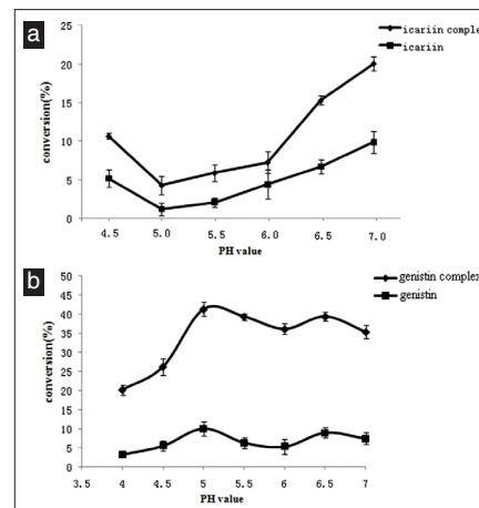
Figure 4: (a). Effect of pH on efficiency of icariin (icariin/ \beta -CD inclusion compounds) hydrolysis The reaction was performed by adding icariin/ \beta -CD inclusion compounds(contains 100mg icariin) or 100mg icariin, 100mg snailase and 10ml glacial acetic acid and sodium acetate anhydrous buffer (pH 4.0, 4.5, 5.0, 5.5, 6.0, 6.5 and 7.0 respectively) at 37°C in digital temperature air bath oscillator for 3h. (b). Effect of pH on efficiency of genistin (genistin/ \beta -CD inclusion compounds) hydrolysis. The reaction was performed by adding genistin/ \beta -CD inclusion compounds (contains 100mg genistin) or 100mg genistin, 100mg cellulase and 10ml glacial acetic acid and sodium acetate anhydrous buffer (pH 4.0, 4.5, 5.0, 5.5, 6.0, 6.5 and 7.0 respectively) at 37°C in digital temperature air bath oscillator for 3h. Values are expressed as mean \pm SD, n = 3
