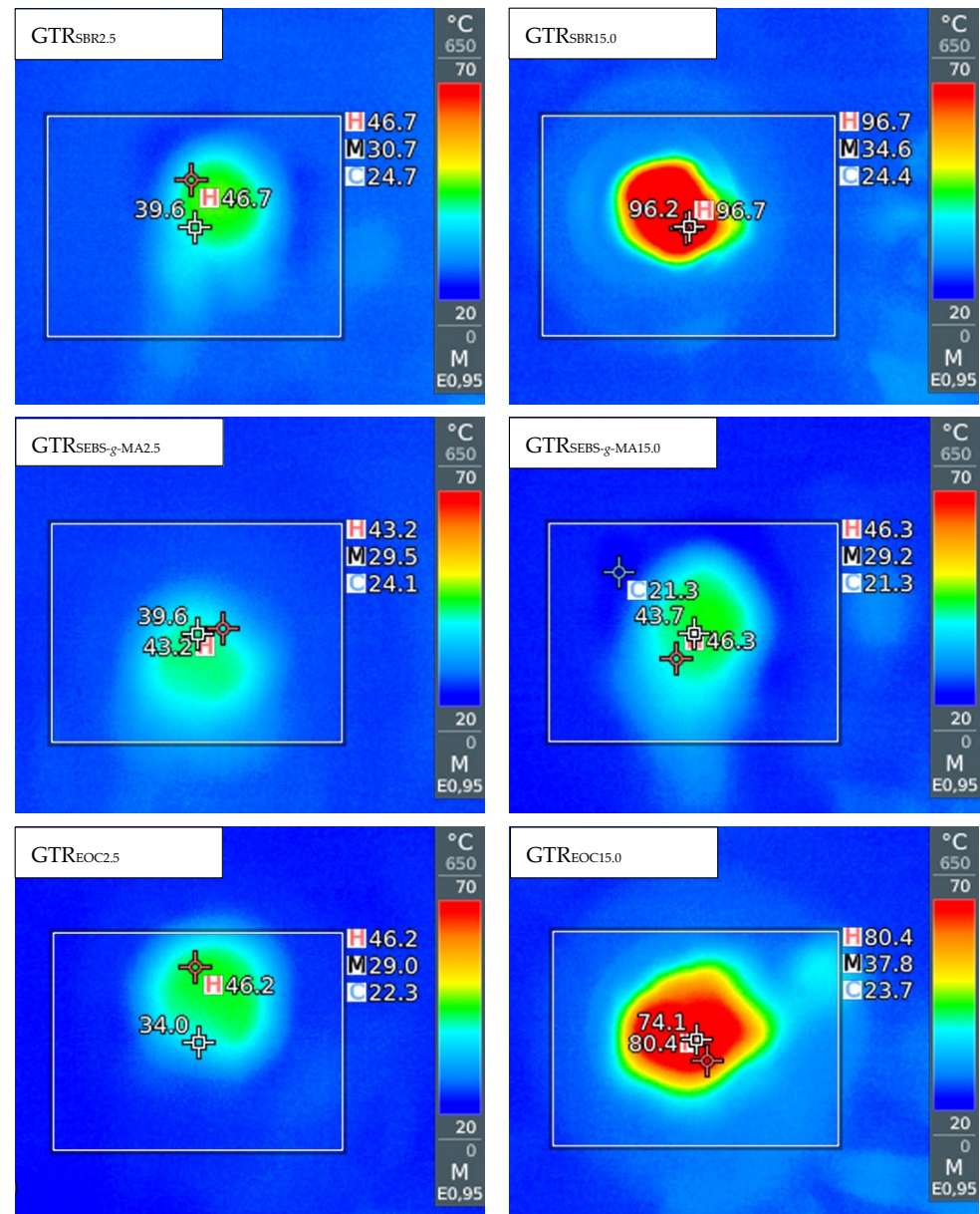
Figure 2. The infrared camera images for selected samples.
