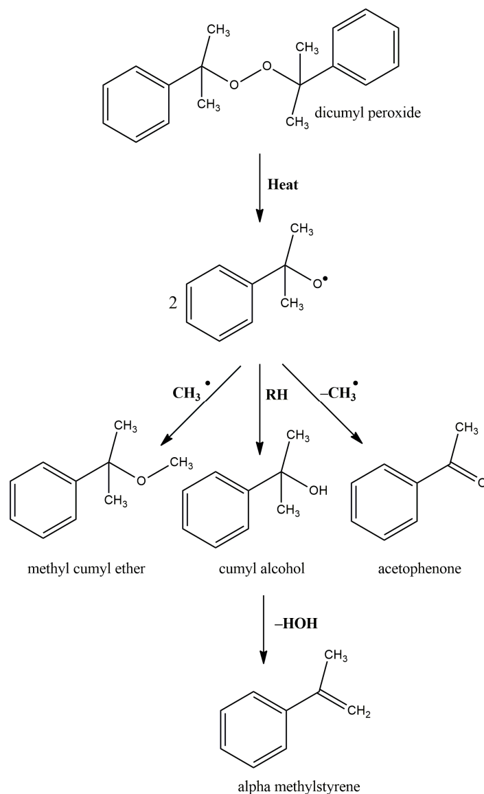
Figure 6. Mechanism of dicumyl peroxide decomposition.
