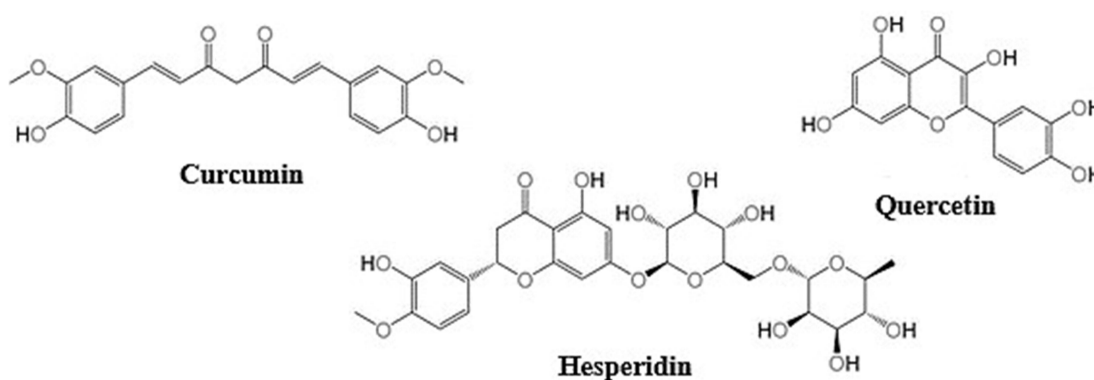
Figure 10 Molecular structure of curcumin, hesperidin and quercetin.
