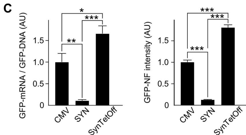
Fig 1. Efficient gene-transduction with AAV-SynTetOff vector in vitro . (A) Construction of the vector plasmids, pAAV2-CMV-GFP-BGHpA, pAAV2-SYN-GFP-BGHpA, and pAAV2-SynTetOff-GFP. (B) One week after infection of Neuro-2a cells with AAV2/1-CMV-GFP-BGHpA, AAV2/1-SYN-GFP-BGHpA, and AAV2/1-SynTetOff-GFP, GFP-NF intensities were measured in the infected cells (outlined by dotted lines with ImageJ). (C) The gene-transduction efficiency with AAV2/1-CMV-GFP-BGHpA, AAV2/1-SYN-GFP-BGHpA, or AAV2/1-SynTetOff-GFP was examined quantitatively. The GFP-mRNA/GFP-DNA ratio and the GFP-NF intensity of cells infected with AAV2/1-CMV-GFP-BGHpA were standardized as 1 arbitrary unit (AU). A qRT-PCR assay revealed that GFP-mRNA expression was 1.7- and 15.6-fold higher with AAV2/1-SynTetOff-
