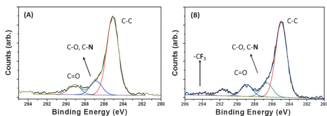
Figure 2. XPS C1s of a 3:1 mixture of octylphosphonic and 1,2-quinone-terminated surface A) before SPOCQ reaction ( S3 ) and B) after SPOCQ reaction ( S4 ) with BCN derivative 1 (3 mM in dichloroethane at 30 °C, 8 h).
