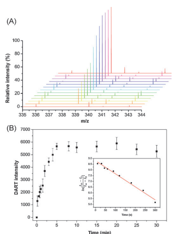
Figure 4. A) Relative intensity for the MS tag at different reaction times (from 0 to 15 min). B) Normalized intensity for MS tag for the SPOCQ reaction. Inset: Plot of \ln[(I_\infty - I_t)/(I_\infty - I_0)] vs. time, used to obtain the rate constant.
