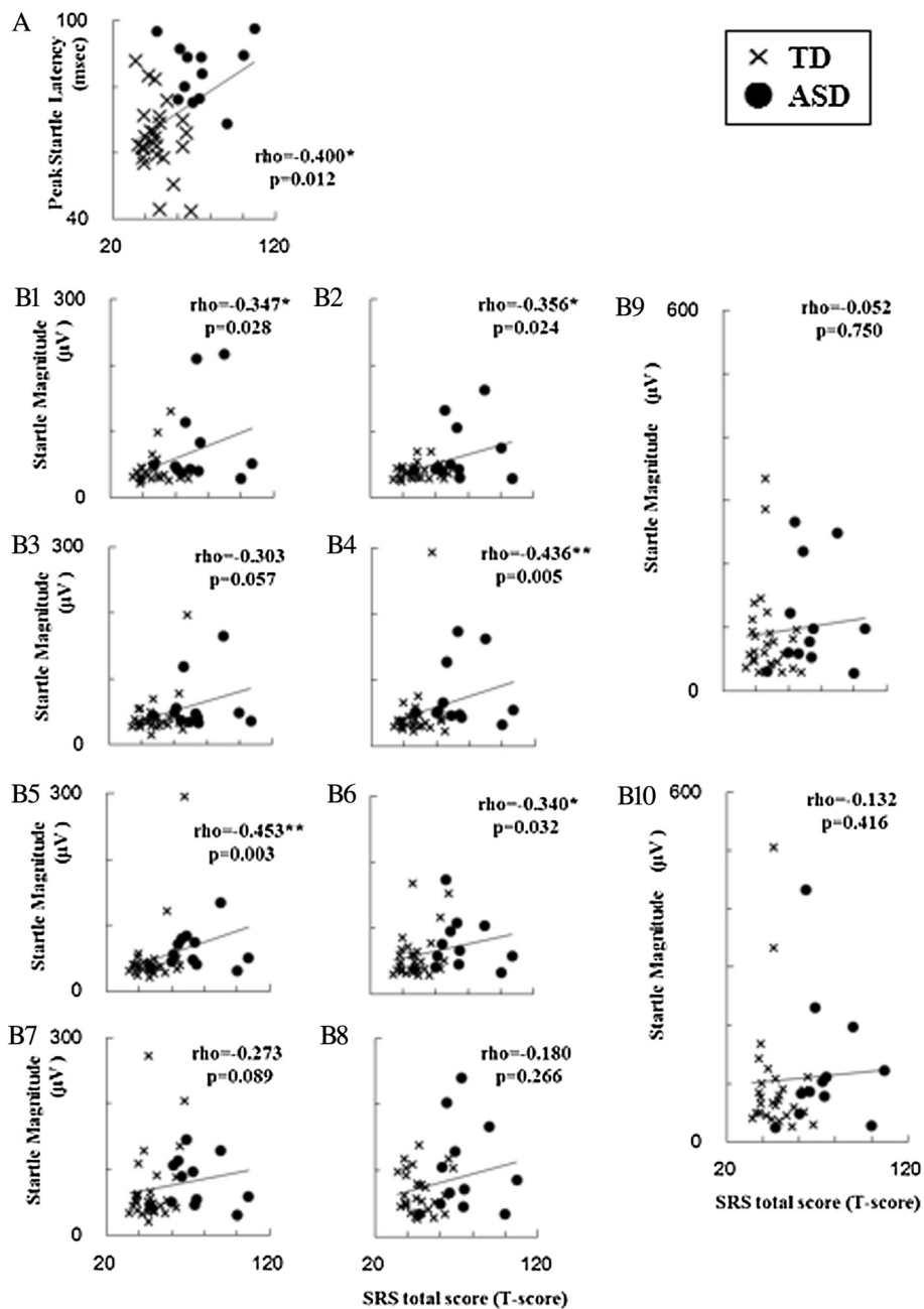
Figure 2 Scatterplots of startle measures by T-score of Social Responsiveness Scale (SRS) total score. (A) PSL for T-score of the SRS total score. (B1), (B2), (B3), (B4), (B5), (B6), (B7), (B8), (B9) and (B10) represent ASR65, ASR70, ASR75, ASR80, ASR85, ASR90, ASR95, ASR100, ASR105 and ASR110, respectively, for T-score of the SRS total score. Variables are rho. ASR65, ASR70, ASR75, ASR80, ASR85, ASR90, ASR95, ASR100, ASR105 and ASR110 are designated as the average startle eyeblink magnitude at stimulus intensities of 65, 70, 75, 80, 85, 90, 95, 100, 105 and 110 dB, respectively. n = 40 (ASD, n = 12; TD, n = 28). Spearman's rank order correlation; *P < 0.05; **P < 0.01. ASD, autism spectrum disorders; ASR, acoustic startle reflex; PSL, peak startle latency of acoustic startle reflex; SRS, Social Responsiveness Scale; TD, typical development.
