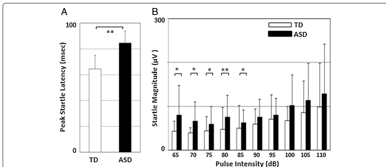
Figure 1 Comparison of startle measures between children with autism spectrum disorders (ASD) and typical development (TD). (A) Comparison of PSL between ASD and TD (ASD, n = 12 ; TD, n = 28 ). (B) Comparison of startle magnitude at each stimulus intensity between ASD and TD (ASD, n = 12 ; TD, n = 28 ). The figures show the means and the error bars show the standard deviation. Mann-Whitney U test; * P < 0.05 ; ** P < 0.01 . ASD, autism spectrum disorders; PSL, peak startle latency; TD, typical development.
