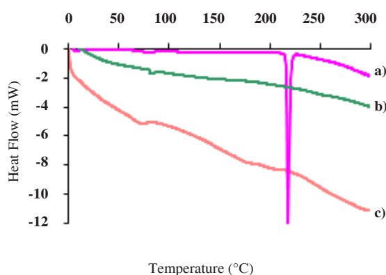
Figure 2. DSC thermograms: a) pure drug, b) E-RSPO nanoparticles loaded with LMG, c) E-RSPO
