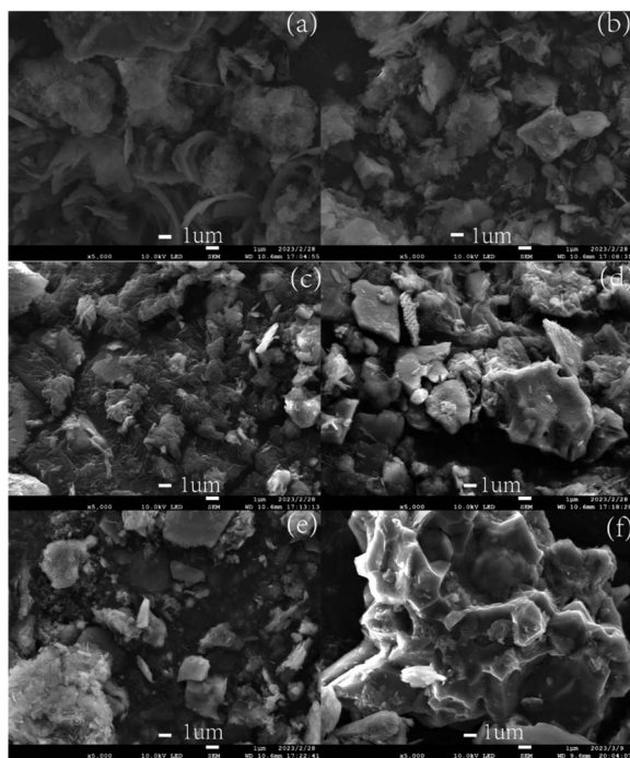
Fig. 7 The microscopic morphological changes of dredged sediment surface with the addition of St-CTA as (a) 0 \text{ mg g}^{-1} TSS, (b) 3 \text{ mg g}^{-1} TSS, (c) 6 \text{ mg g}^{-1} TSS, (d) 9 \text{ mg g}^{-1} TSS, (e) 12 \text{ mg g}^{-1} TSS, and (f) 18 \text{ mg g}^{-1} TSS.
