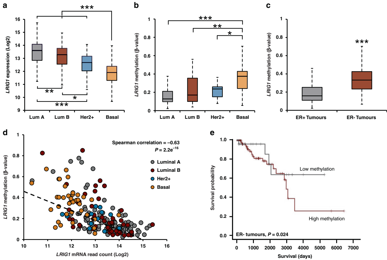
Fig. 2 LRIG1 DNA methylation negatively regulates LRIG1 mRNA expression. a Boxplot depicting LRIG1 mRNA expression (read count) in Luminal A ( n = 439 ), Luminal B ( n = 118 ), Her2 + ( n = 37 ) and Basal ( n = 112 ) breast tumours (data from TCGA). b Boxplot depicting LRIG1 \beta -values in Luminal A ( n = 110 ), Luminal B ( n = 46 ), Her2 + ( n = 14 ) and Basal ( n = 41 ) breast tumours (data from TCGA). c Boxplot depicting LRIG1 \beta -values in ER-positive ( n = 565 ) and ER-negative ( n = 167 ) breast tumours (data from TCGA BRCA). d Scatter plot of patient-matched LRIG1 mRNA read count and LRIG1 \beta -values in breast tumour samples ( n = 204 ). Black dotted line indicates linear regression (data from TCGA BRCA). e Kaplan–Meier plot of overall survival as a function LRIG1 methylation in ER-negative tumours. Patients were segregated into groups based on ER \alpha status and LRIG1 \beta -value in their primary tumour (high methylation/ER-negative: n = 135 , low methylation/ER-negative: n = 32 ) (data from TCGA BRCA). * P < 0.05 , ** P < 0.01 and *** P < 0.001 , respectively; Tukey’s HSD ( a , b ), Student’s t test ( c ), Spearman correlation test ( d ), log-rank test ( e ).
