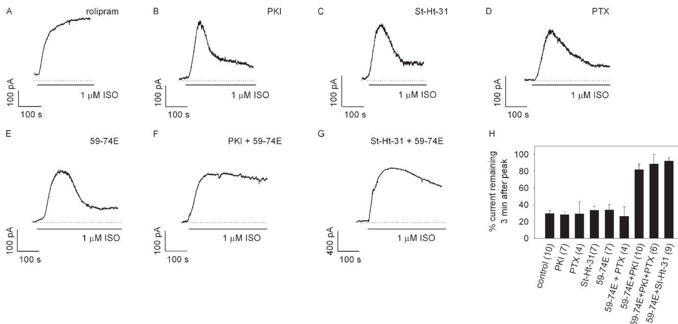
Figure 3. Pharmacological profiling of the molecular mechanisms underlying transient isoproterenol-induced cAMP signals. Responses were elicited by exposure of CNG channel-expressing cells to 1 μM isoproterenol. (A) The decline in the cAMP transients was abolished when 10 μM rolipram (a PDE4 inhibitor) was included in the patch pipette. The decline in the response remained largely intact when 20 nM PKI (a PKA inhibitor, B) or 10 μM St-Ht31 (an AKAP-PKA disruptor, C) were included in the patch pipette, indicating the PKA was not solely responsible for the decline in the signal. (D) An 18–24-h pretreatment with PTX (an inhibitor of G_i ) had little effect on the overall kinetics of the signal. (E) 3 μM 59-74E (a GRK inhibitor) did not prevent the decline in the cAMP transients. However, the decline in the response was largely eliminated when both PKI and 59-74E (F) or St-Ht31 and 59-74E (G) were included in the patch pipette. (H) Data were quantified by measuring the percentage of current remaining 3 min after the peak current.
