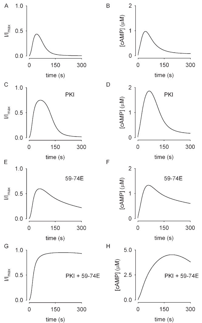
Figure 6. Mathematical simulations of the system described by the schematic in Fig. 5. Panels on left depict the signal being measured, panels on right depict the underlying cAMP signals. (A and B) Simulations of normalized current through CNG channels ( I/I_{max} ) due to isoproterenol-induced cAMP signals under control conditions. (C and D) Simulations of isoproterenol-induced currents and cAMP signals in the presence of 20 nM PKI (included in the pipette solution). Including PKI in the pipette solution inhibits PKA-mediated stimulation of PDE activity, allowing increased cAMP levels, but the signal is still transient due to basal PDE4 activity and GRK-mediated receptor desensitization. (E and F) Simulations describing the effect of GRK inhibition (3 \mu M 59-74E) on isoproterenol-induced signals. The signals are still transient due to PKA-mediated stimulation of PDE4 activity. (G and H) Simulations of currents and cAMP signals when both PKA and GRK activity are inhibited (with PKI and 59-74E). Inhibiting receptor desensitization and the stimulation of PDE4 activity prevents the decay of isoproterenol-induced signals.
