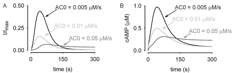
Figure 8. Simulated effects of increased basal AC activity on \beta 2AR-mediated cAMP signaling. (A and B) Increasing basal adenylyl cyclase activity from control levels of 0.005 \mu\text{M/s} to 0.05 \mu\text{M/s} increased both the basal PKA and PDE activities, in essence priming the negative feedback loop. The effects of this priming phenomena were (B) smaller cAMP signals leading to (A) decreased peak currents through CNG channels. In addition, the overall kinetics of the signal were slowed with increased basal AC activity, and, at the highest basal AC activity shown, were no longer transient.
