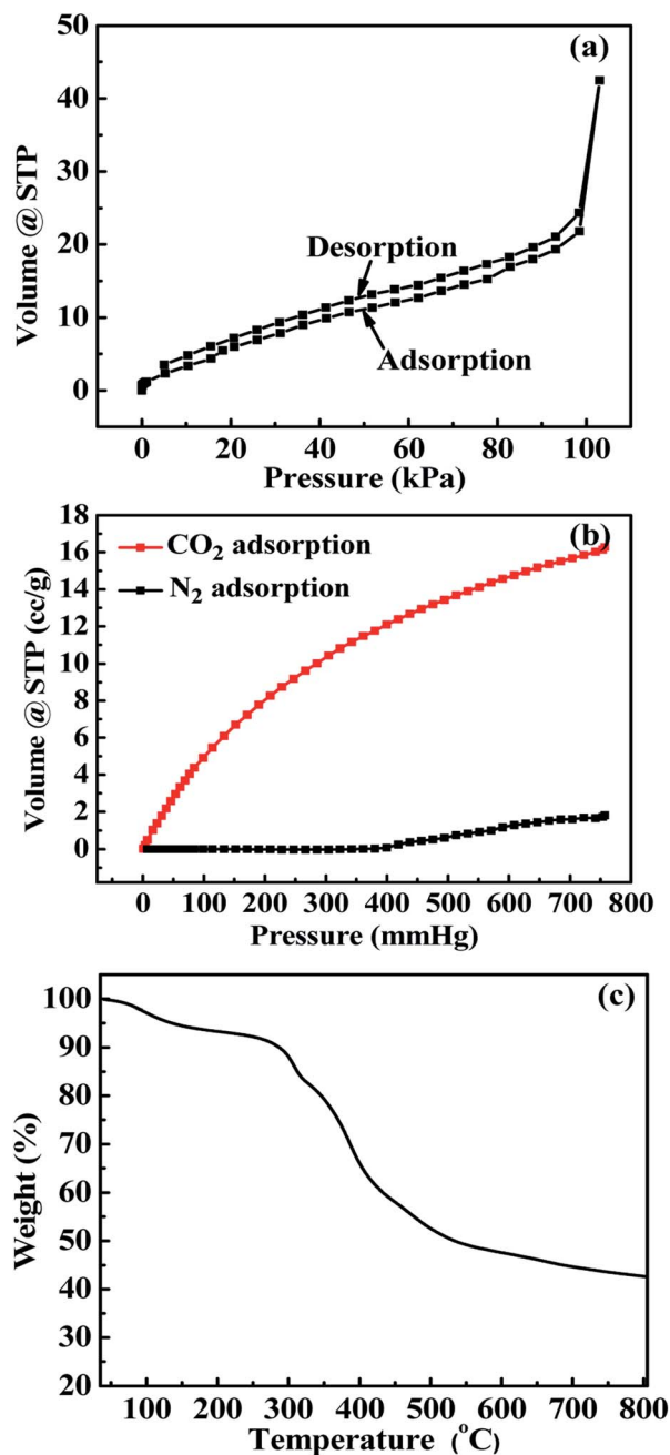
Fig. 3 (a) \text{N}_2 adsorption-desorption isotherms; (b) \text{CO}_2 and \text{N}_2 adsorption capacities; and (c) TGA plot of Co(azpy) prepared by microwave method.
