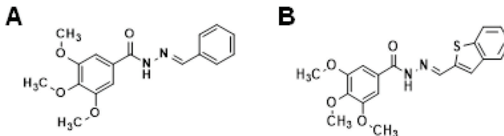
Figure 2 - Combrestatin A-4 analogs. (A) LASSBio-1586. (B) LASSBio-1920.
