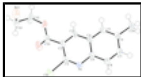
Fig. 1. (Farrugia, 1997) the structure of the title compound with the atomic labelling scheme. Displacement are drawn at the 50% probability level.
