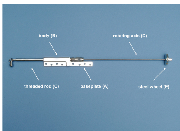
Figure 1 Tensioning device with holes for locking screws through the baseplate (A). Through axial rotation on the steel wheel (E) the threaded rod (C) exits the opposite side of the body (B) and thereby elongates the muscle tendon unit, which is fixed to the end of the threaded rod by sutures.
