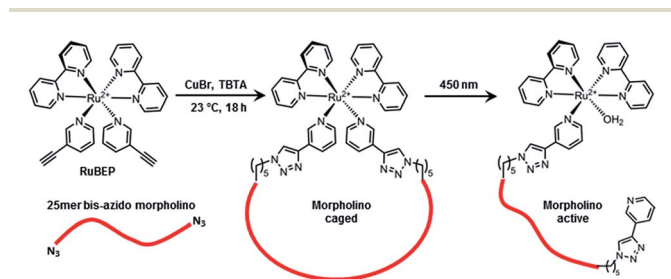
Scheme 1 RuBEP photolinker conjugated with 25mer bis-azido morpholino formed "caged" antisense MO; subsequent 450 nm irradiation restored biologically active MO.
