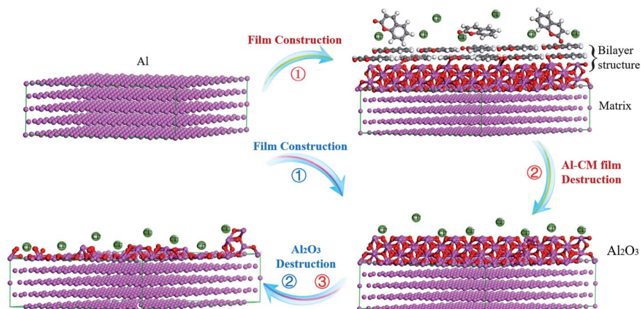
Fig. 10 Schematic diagrams of the corrosion inhibition mechanism of coumarin in chloride-containing environment.
