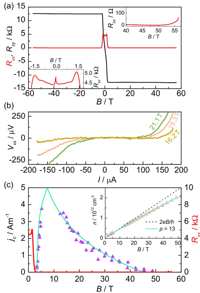
Figure 3. Giant quantum Hall plateaus. Pulsed magnetic field measurements of the quantum Hall effect in epitaxial graphene on SiC at T=2 K as observed in the longitudinal resistance ( R_{xx} , red) and Hall resistance ( R_{xy} , black) showing an exceptionally wide ( \sim 50 T) \nu=2 plateau. Upper inset: The end of the plateau at B > 50 T. Lower inset: R_{xx} at low magnetic fields showing clear Shubnikov-de Haas oscillations and weak localisation. (b) Examples of high speed I - V_{xx} traces taken during a single pulsed magnetic field measurement, showing that clear quantum Hall breakdown behaviour is observed. (c) Magnetic field dependence of the breakdown current (purple triangles) for the \nu=2 plateau and a best fit (solid line) using equations (1) and (6) with the power p=13 . The red line shows the longitudinal resistivity and the inset shows the corresponding magnetic field dependent carrier density.
