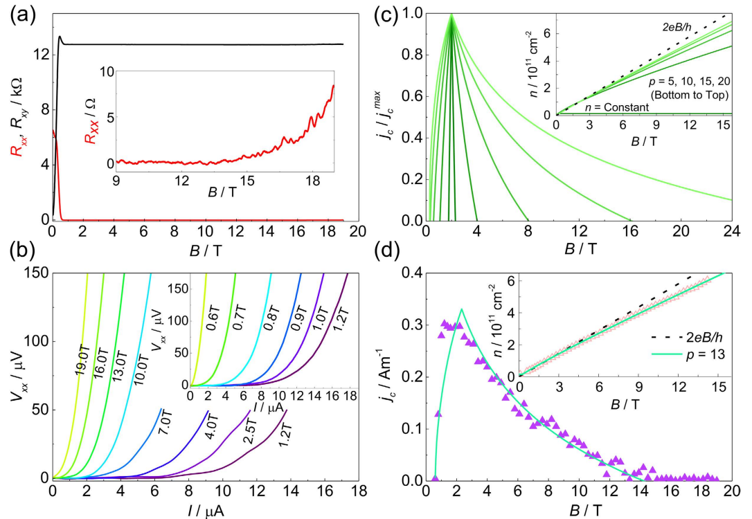
Figure 1. Quantum Hall effect in ultra-low carrier density epitaxial graphene. (a) Continuous field measurements of the quantum Hall effect at 2 K using a constant measurement current of 1 \mu A in an epitaxial graphene on SiC sample with the zero field carrier density reduced to 1.5 \times 10^{10} \text{ cm}^{-2} by corona discharge at room temperature. Inset: an expanded plot of R_{xx} towards the end of the plateau. (b) I-V traces indicating the onset of the quantum Hall breakdown for the high magnetic field side of the plateau and inset, for the low field side. (c) Theoretical dependence of the breakdown current for the \nu=2 quantum Hall plateau using equations (1) and (6) with B_0=0.3 \text{ T} and B_c=2.0 \text{ T} . A set of dependences are shown with the power, p , chosen as 5, 10, 15, and 20. The traditional triangular dependence of breakdown current on magnetic field for constant n becomes stretched and asymmetric as the carrier density tends towards an almost linear dependence on magnetic field. The inset shows the corresponding field dependent carrier densities. (d) Magnetic field dependence of the breakdown current (purple triangles) for the \nu=2 plateau and a best fit (solid line) using equations (1) and (6) with the power p=13 . The inset shows the corresponding magnetic field dependent carrier density.
