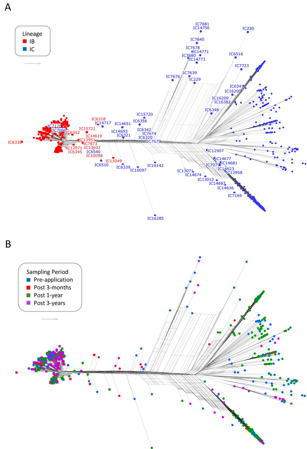
Fig 1. Patterns of reticulate evolution for 815 A. flavus isolates. A. Network splits tree graph highlighting in color membership of each isolate in lineage IB (red) or IC (blue) as determined from phylogenetic, admixture and cluster analysis. The terminal most splits include isolates that are representative of the clonal component of each lineage and isolates arising predominantly from intra-lineage recombination events. Putative hybrids resulting from recombination between lineages IB and IC are labeled and occupy mostly interior positions in the network. Putative hybrid strains are highly divergent and contain varying proportions of both lineages in their genetic background as shown in Fig 2. B. Overlay of sampling period on the network in A showing that inter-lineage recombination is a common feature of each sampling period. The network shows greater genetic heterogeneity within lineage IC compared to IB and that post 3-year samples were predominantly sampled from lineage IB. The branches in the network are drawn to scale and the scale bar represents 0.01 substitutions per site.
