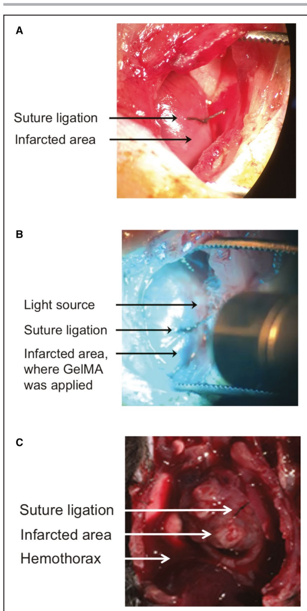
Figure 3. Experimental myocardial infarction (MI) and gelatin methacryloyl (GelMA) photo-crosslinking in situ.
