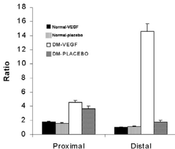
Figure 3 Ratio of smooth muscle actin positive cells in the ischemic to nonischemic limb in the proximal and distal limb segments. Each group contains 4 or 5 animals. Ratio and P Values: Proximal: VEGF arm (1.8) Vs. Placebo (1.5) p < 0.05, Vs both DM arms p < 0.001, Normal placebo Vs. both DM arms p < 0.001, DM VEGF (4.5) Vs DM-Placebo (3.6) p < 0.05. Distal: VEGF arm (1.0) Vs. Placebo (1.1) p = NS, Vs DM-VEGF p < 0.001, Vs. DM-Placebo p < 0.01, DM VEGF (14.6) Vs DM-Placebo (1.7) p < 0.01.
