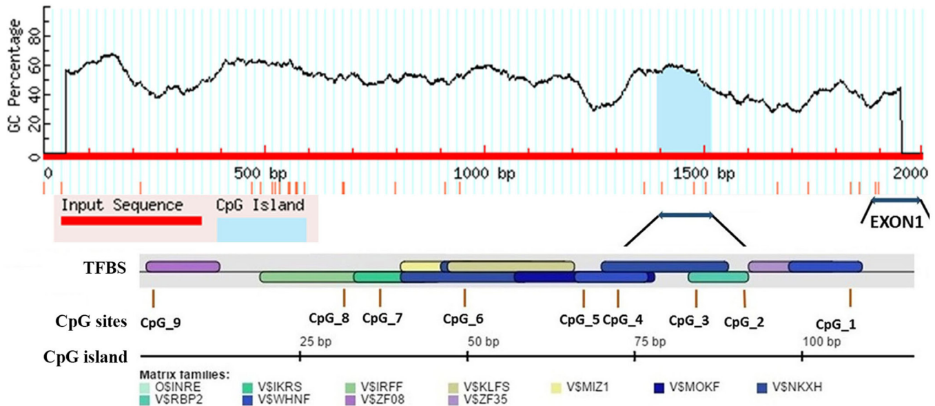
Figure 1. Bioinformatic analyses of the CpG island of porcine cluster of differentiation 4 protein ( CD4 ) gene upstream -2 kb and exon one region. This figure only demonstrated 11 of 15 TFBS containing CpG sites. TFBS, transcription factor binding sites; Matrix Families: similar and/or functionally related TFBS are grouped into so-called matrix families.
