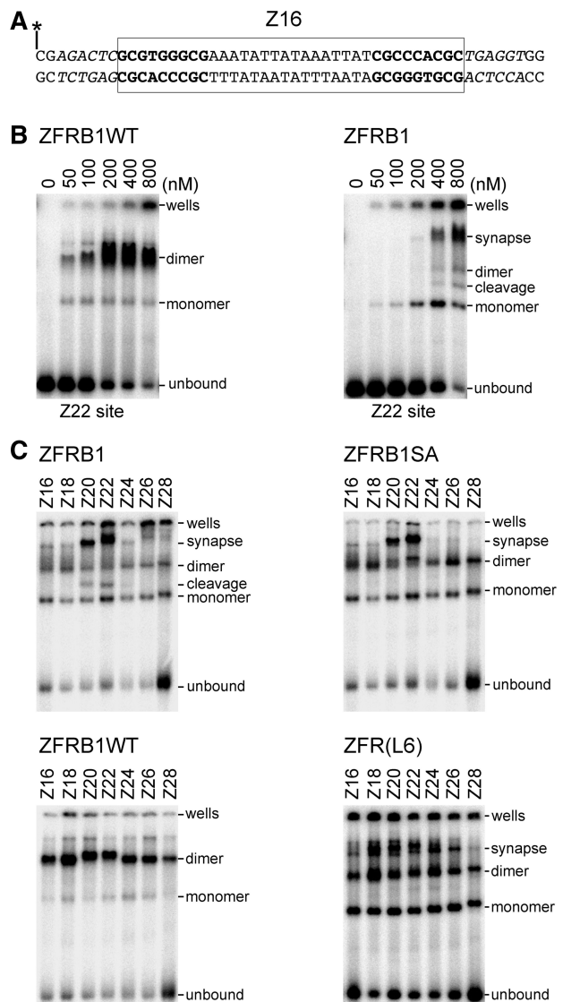
Figure 6. Binding and synthesis of Z-sites by ZFRs. (A) The substrates used for the bandshift experiments. All the substrates are exactly 50 bp, with a centrally positioned Z-site. The diagram shows the Z16 site (boxed), with the motifs recognized by the Zif268 domains in bold. The longer Z-sites are similar except that the core sequence is longer (Figure 2C), and one or more of the immediately flanking basepairs at each end of the site (in italics) is deleted. The asterisk indicates the position of the 5'- 32 P label. (B) Binding of the Z22 site by varying concentrations of ZFRB1WT (left panel) and ZFRB1 (right panel). Estimated ZFR concentrations are indicated above each lane. The band marked 'cleavage' is a labelled half-site cleavage product with a ZFR monomer covalently attached via the active site serine residue; see text for details. (C) Binding of Z-sites (as indicated above the lanes) by ZFRB1 (top left), ZFRB1SA (top right), ZFRB1WT (bottom left) and ZFR(L6) (bottom right).
