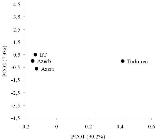
Fig. 2: Principal coordinates plot based on R_{ST} values
