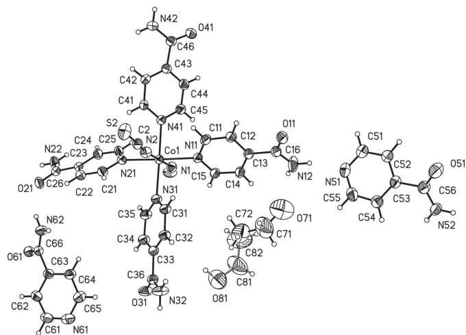
Figure 1 View of the asymmetric unit of the title compound, with atom labelling and displacement ellipsoids drawn at the 50% probability level. The positional disorder of the ethanol molecule is shown by full and open bonds for the two orientations.
