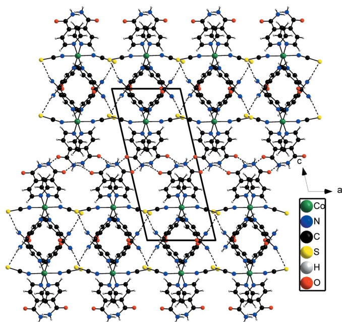
Figure 3 Crystal structure of the title compound in a view along the b axis. Intermolecular hydrogen bonding is shown as dashed lines and the second orientation of the disordered ethanol molecule is omitted for clarity.
