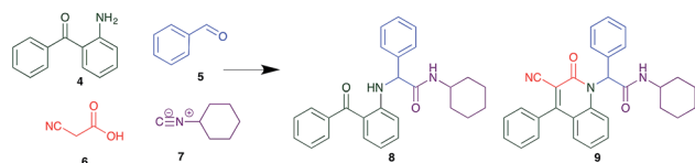
Scheme 1 Reagents and conditions: CH 3 OH, rt.
