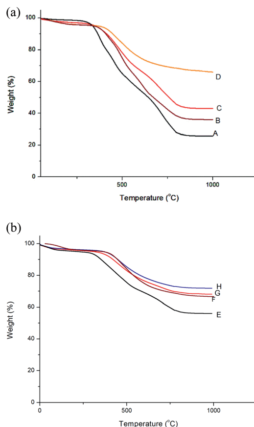
Fig. 9 (a) TGA curves of PIs and Nanocomposites (A) BAPQMCPM-BPADA PI (B) BAPQMCPM-BPADA PI/2%F-silica, (C) BAPQMCPM-BPADA PI/5%F-silica, (D) BAPQMCPM-BPADA PI/10%F-silica. (b) TGA curves of PIs and Nanocomposites (E) BAPQMCPM-BTDA PI, (F) BAPQMCPM-BTDA PI/2%F-silica, (G) BAPQMCPM-BTDA PI/5%F-silica (H) BAPQMCPM-BTDA PI/10% F-silica.
