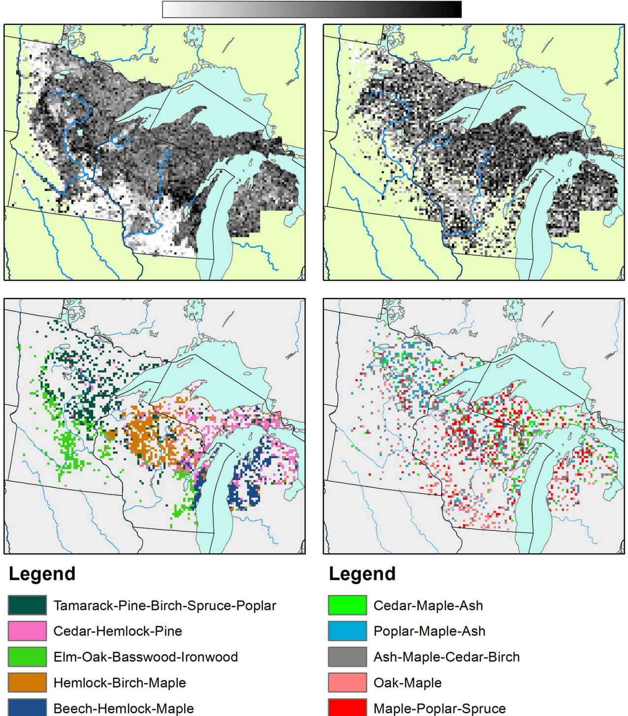
Fig 8. Minimum dissimilarity maps. Distributions of minimum (within dataset) dissimilarities during the PLSS (a) and FIA (b) show spatially structured patterns of dissimilarity, with stronger spatial coherence for the PLS. Lost forests (c) show strong compositional and spatial coherence, and have more taxa with percent composition > 10% than within Novel forests during the FIA era (d). The lost Elm-Oak-Basswood-Ironwood zone lies south of the Tension Zone [16,72], while the other zones lie largely north or east of the Tension Zone. The spatial structure of the novel forests is less well defined.
