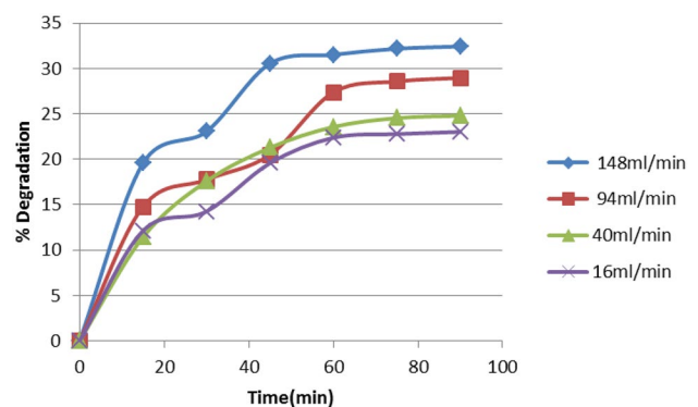
Fig. 7 Effect of flow rate on the photodegradation efficiency of dye
