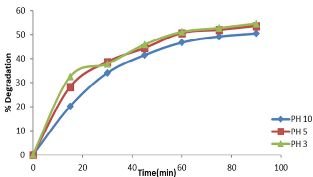
Fig. 8 Percentage dye removal for different solution pH values
