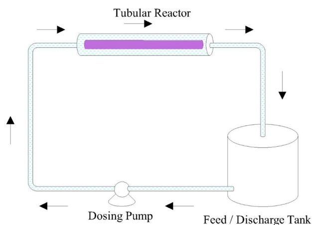
Fig. 1 A schematic diagram for the experimental set-up
