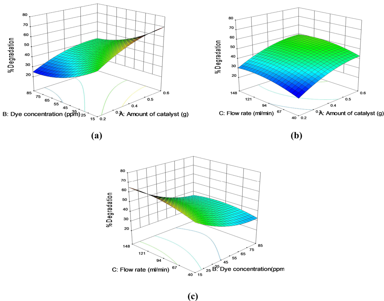
Fig. 11 The response surface plot for the effect of amount of catalyst and dye concentration (a), amount of catalyst and flow rate (b), dye concentration and flow rate (c) on % Degradation
