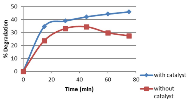
Fig. 9 Comparison of UV- illumination and UV-ZnO NPs catalyzed dye degradation
