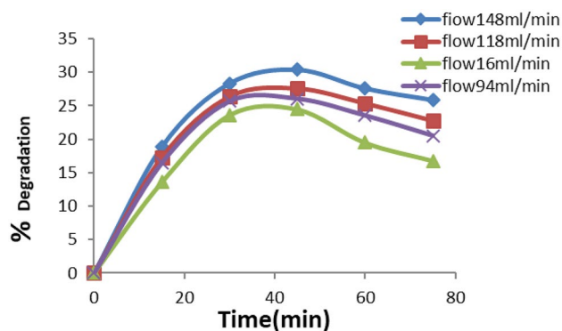
Fig. 3 Effect of flow rate on the photocatalytic degradation of the dye
