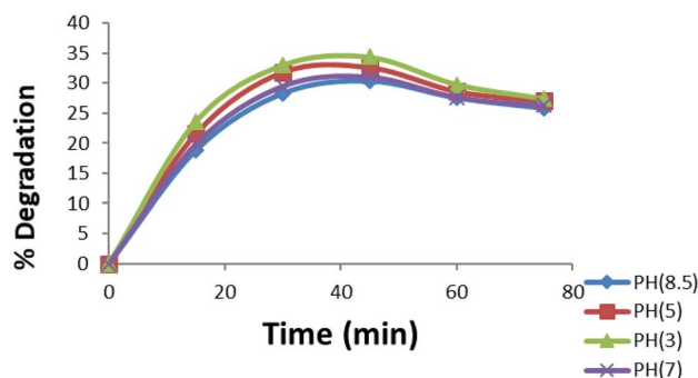
Fig. 4 Effect of pH value on % degradation of 100 ppm dye solution
