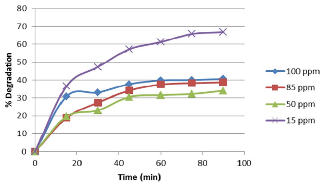
Fig. 5 Effect of initial concentration of EY dye on the degradation efficiency
