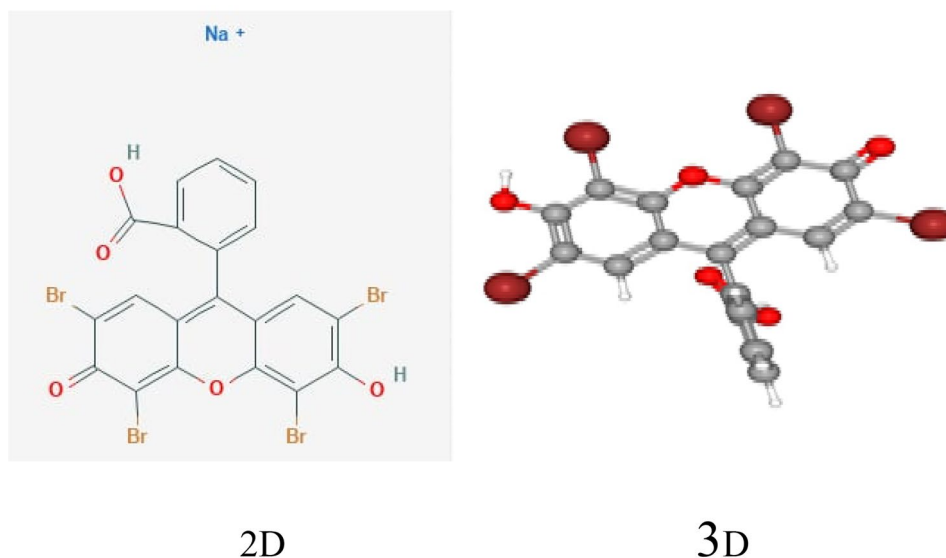
Fig. 2 Structure of Eosin yellow dye
