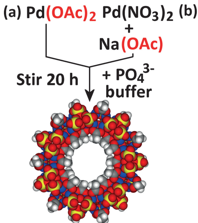
Scheme 1. Two synthetic routes to \{\text{Pd}_{84}\}^{\text{Ac}} using different palladium sources: a) the original route, using palladium acetate; b) a new route, using palladium nitrate.
