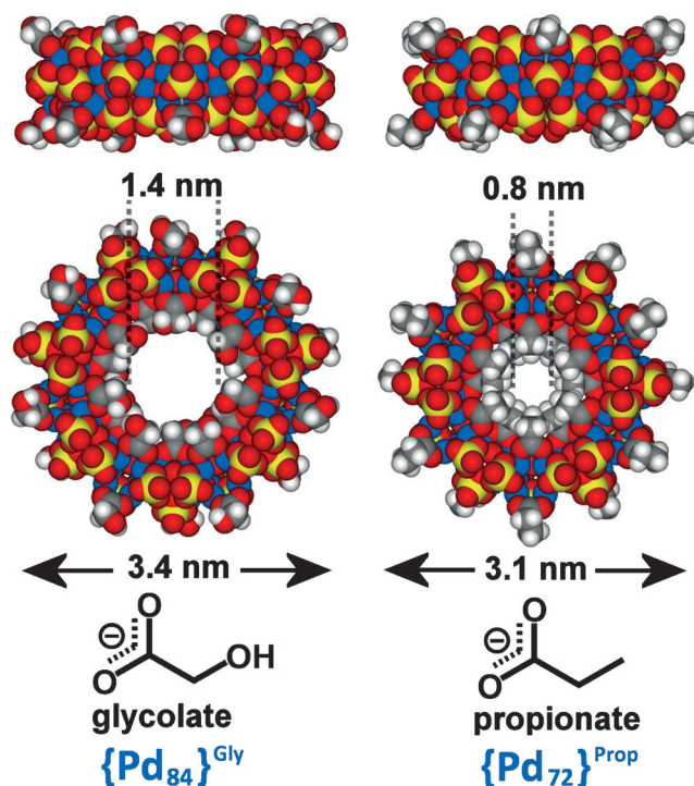
Figure 3. Space filling representation of the two new crystal structures of \{\text{Pd}_{84}\}^{\text{Gly}} (left) and \{\text{Pd}_{72}\}^{\text{Prop}} (right), with the corresponding overall and inner cavity diameters. Key: Pd, blue; O, red; P, yellow; C, grey. Hydrogen atoms omitted for clarity.
