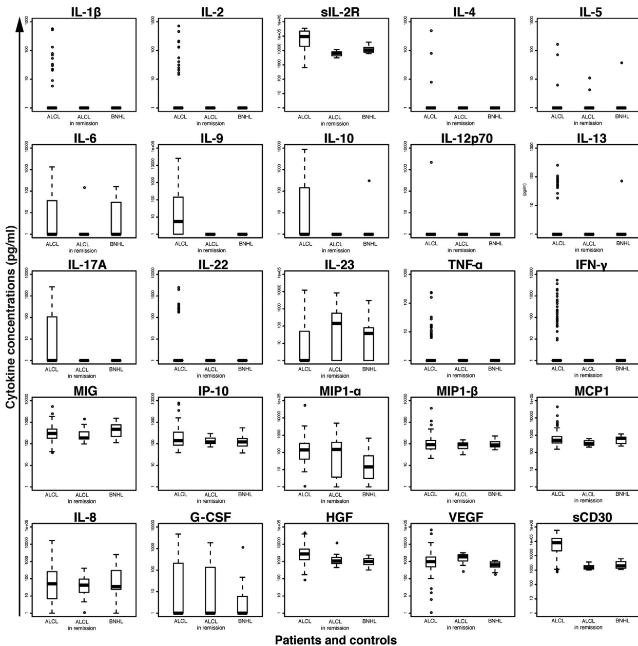
Figure 1. Cytokine levels in patients with anaplastic lymphoma kinase-positive anaplastic large cell lymphoma and controls. Logarithmic representation of cytokine levels in pg/mL for 119 ALCL patients at the time of diagnosis, 15 ALCL patients in remission and 11 patients with B-cell non-Hodgkin lymphoma (B-NHL).
