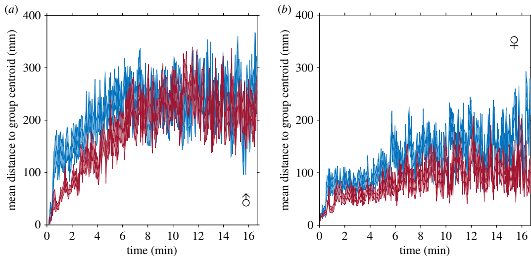
Figure 1. Mean ( \pm 1 s.e.) distance individuals were from the group's centroid for shoals of eight (a) male or (b) female fish. Shoals from high predation environments are shown in red and shoals from low predation environments are shown in blue.
